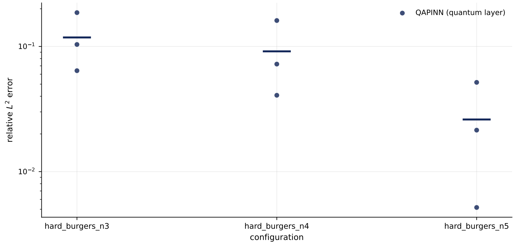
Per-seed results (3 seeds) - dot = seed, bar = mean
